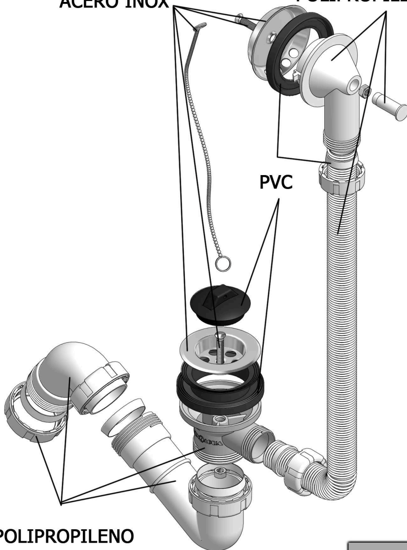
DESPIECE
