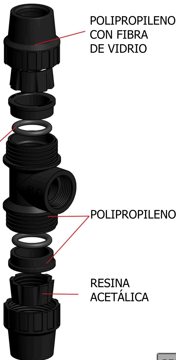
DESPIECE
