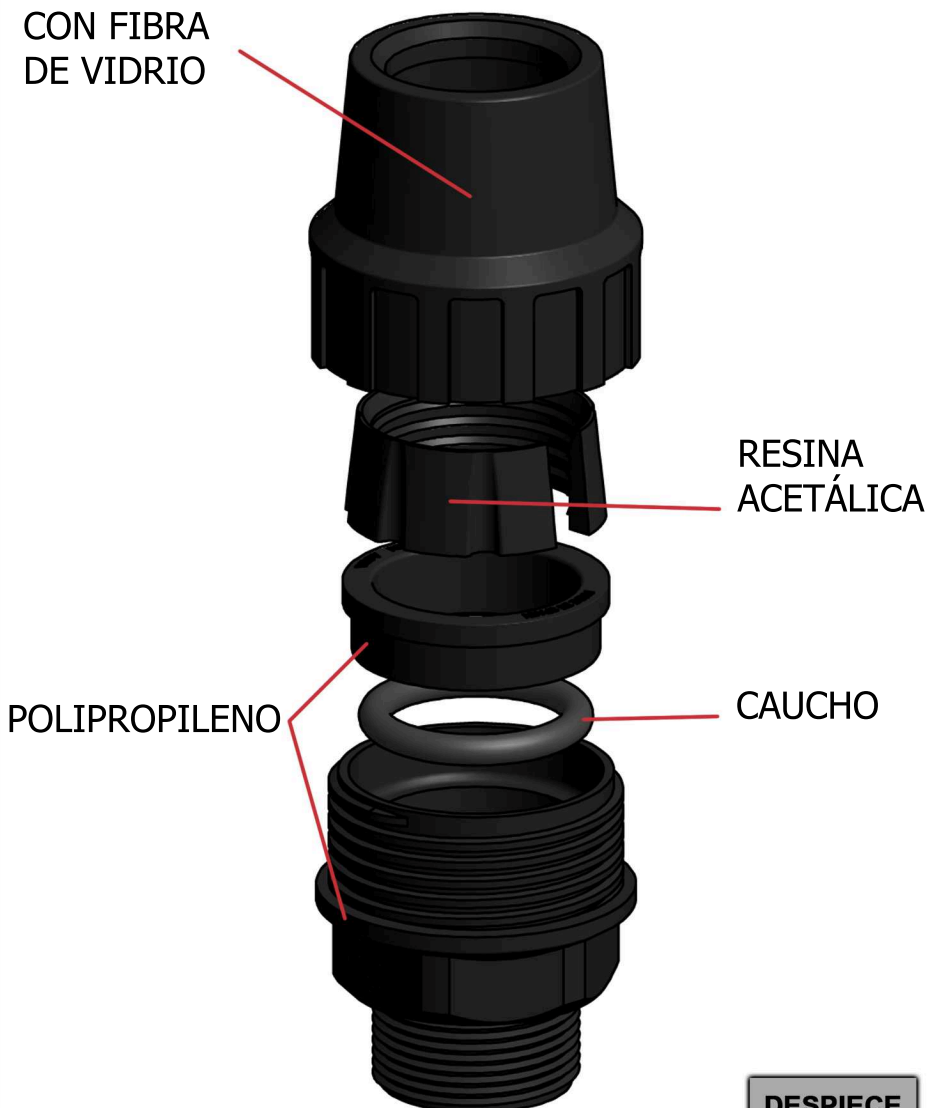
DESPIECE
