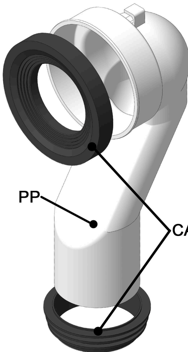
DESPIECE
