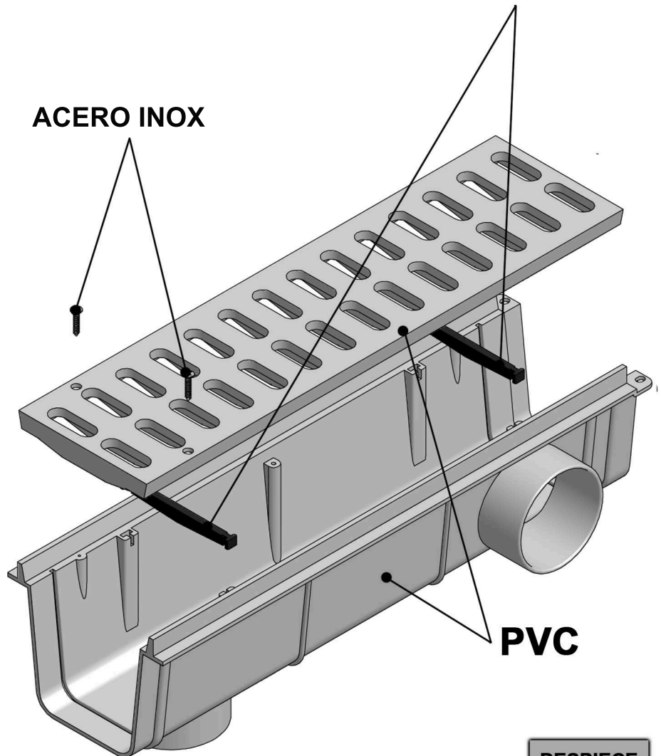
DESPIECE
